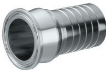
TC - Tri-Clamp®
